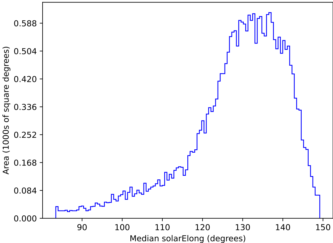
ddf_loaded_half_fl1_v3.4_10yrs All sky i band: Median solarElong
