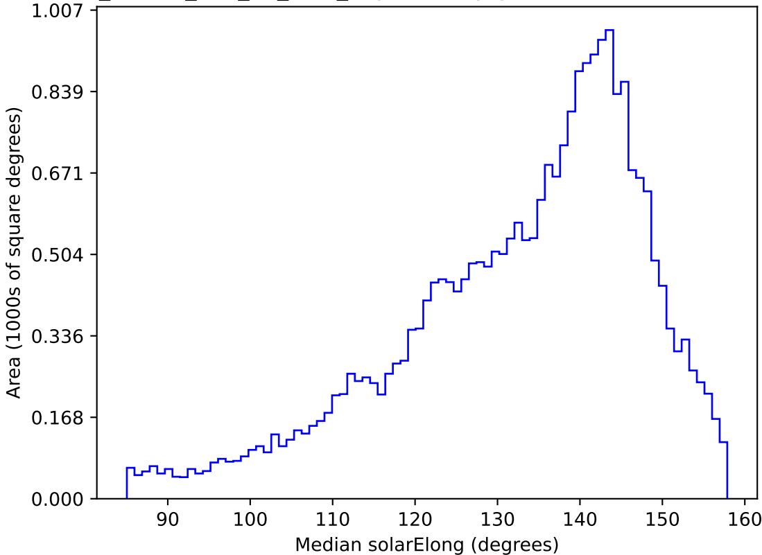
ddf_loaded_half_fl1_v3.4_10yrs All sky g band: Median solarElong
