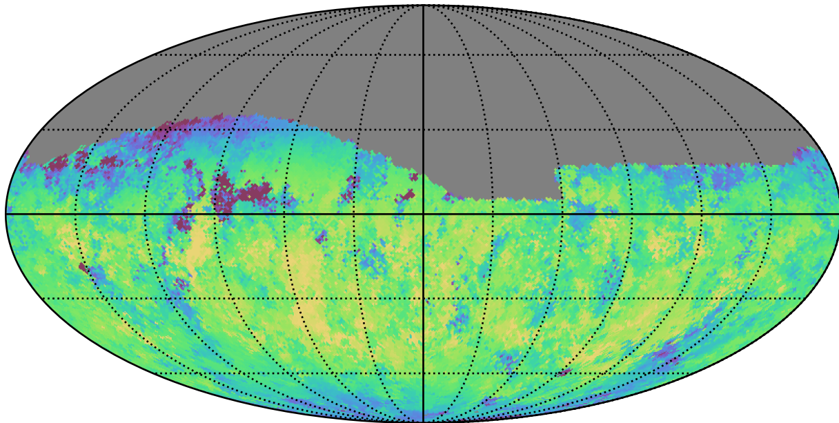
ddf_loaded_half_fl1_v3.4_10yrs Yr 1 z band: Median skyBrightness
