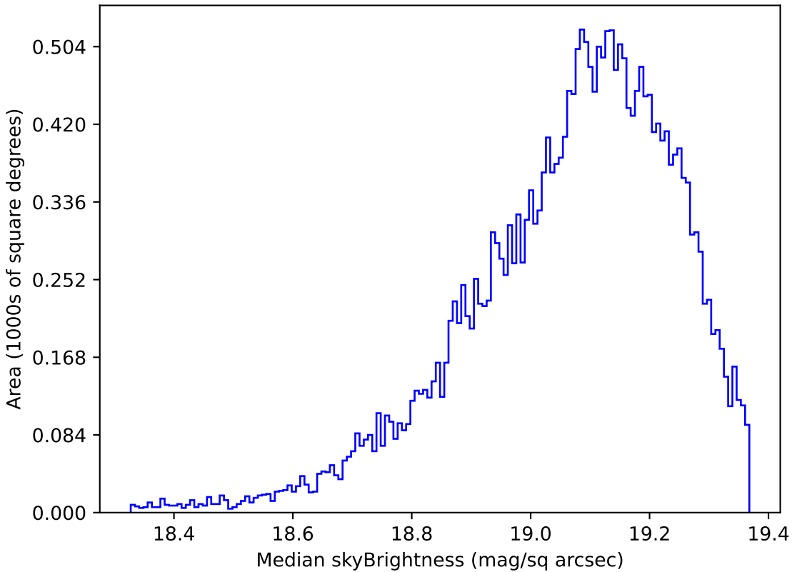
ddf_loaded_half_fl1_v3.4_10yrs Yr 1 z band: Median skyBrightness
