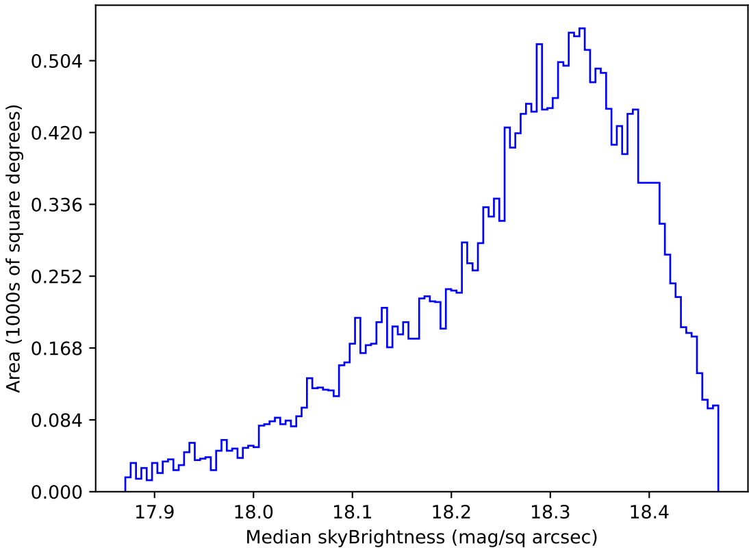
ddf_loaded_half_fl1_v3.4_10yrs Yr 1 y band: Median skyBrightness
