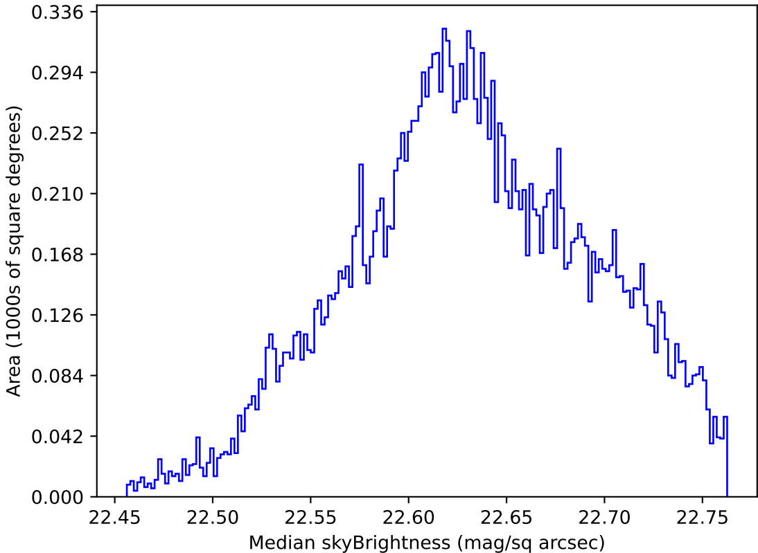
ddf_loaded_half_fl1_v3.4_10yrs Yr 1 u band: Median skyBrightness
