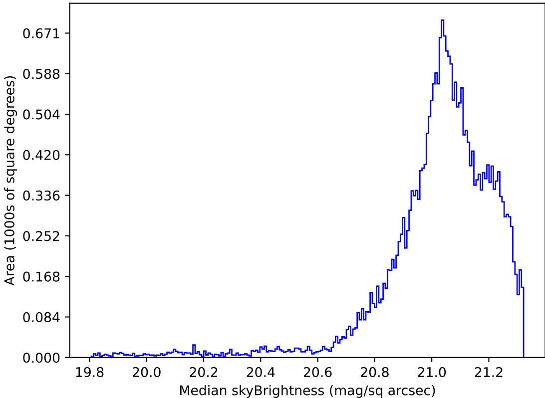
ddf_loaded_half_fl1_v3.4_10yrs Yr 1 r band: Median skyBrightness
