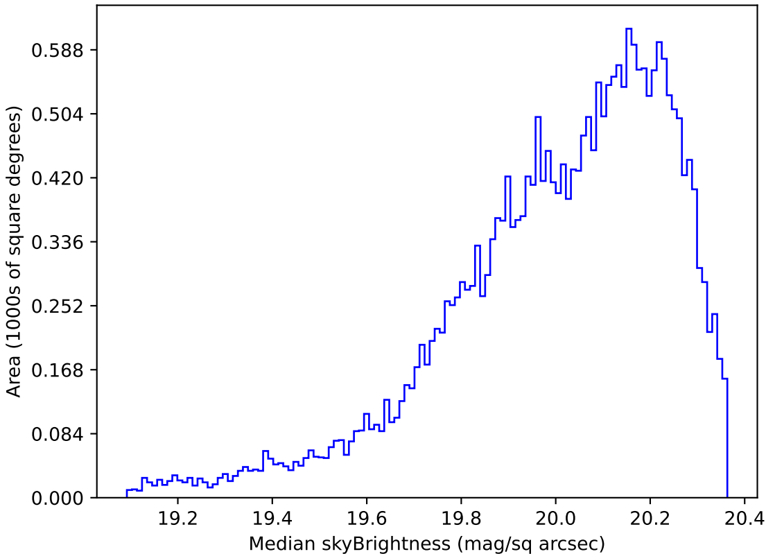
ddf_loaded_half_fl1_v3.4_10yrs Yr 1 i band: Median skyBrightness
