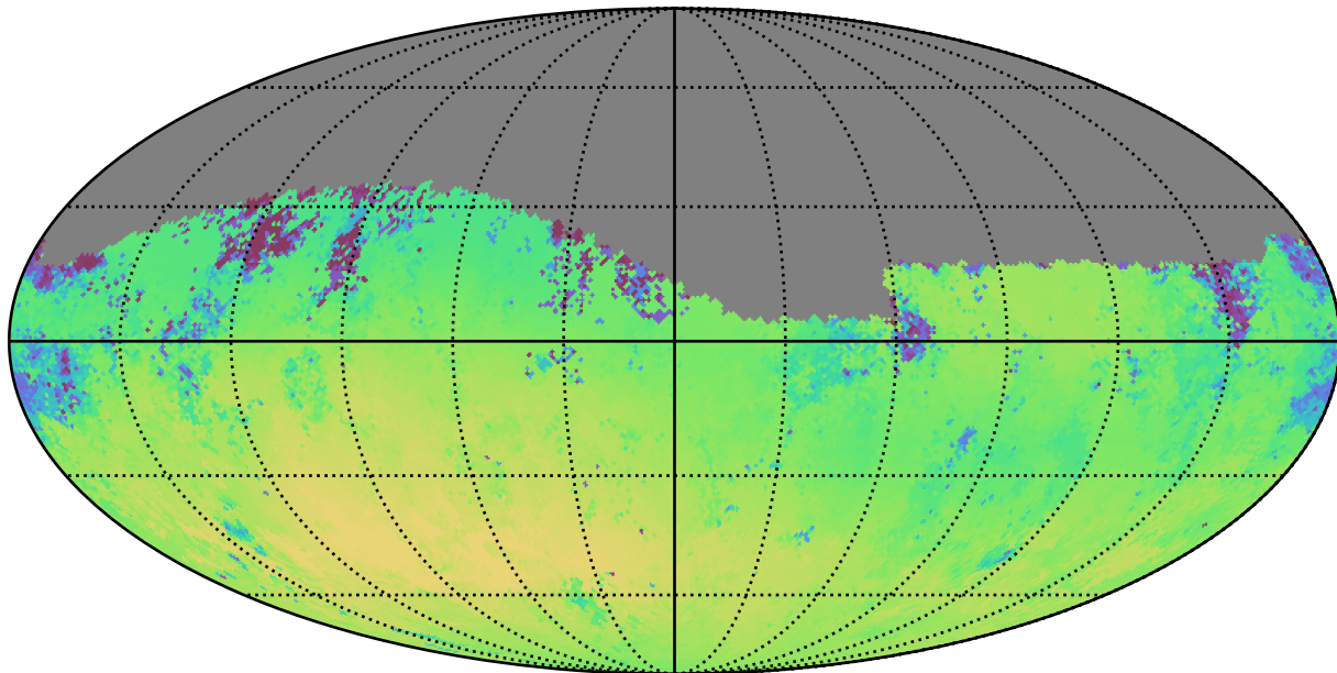
ddf_loaded_half_fl1_v3.4_10yrs Yr 1 g band: Median skyBrightness
