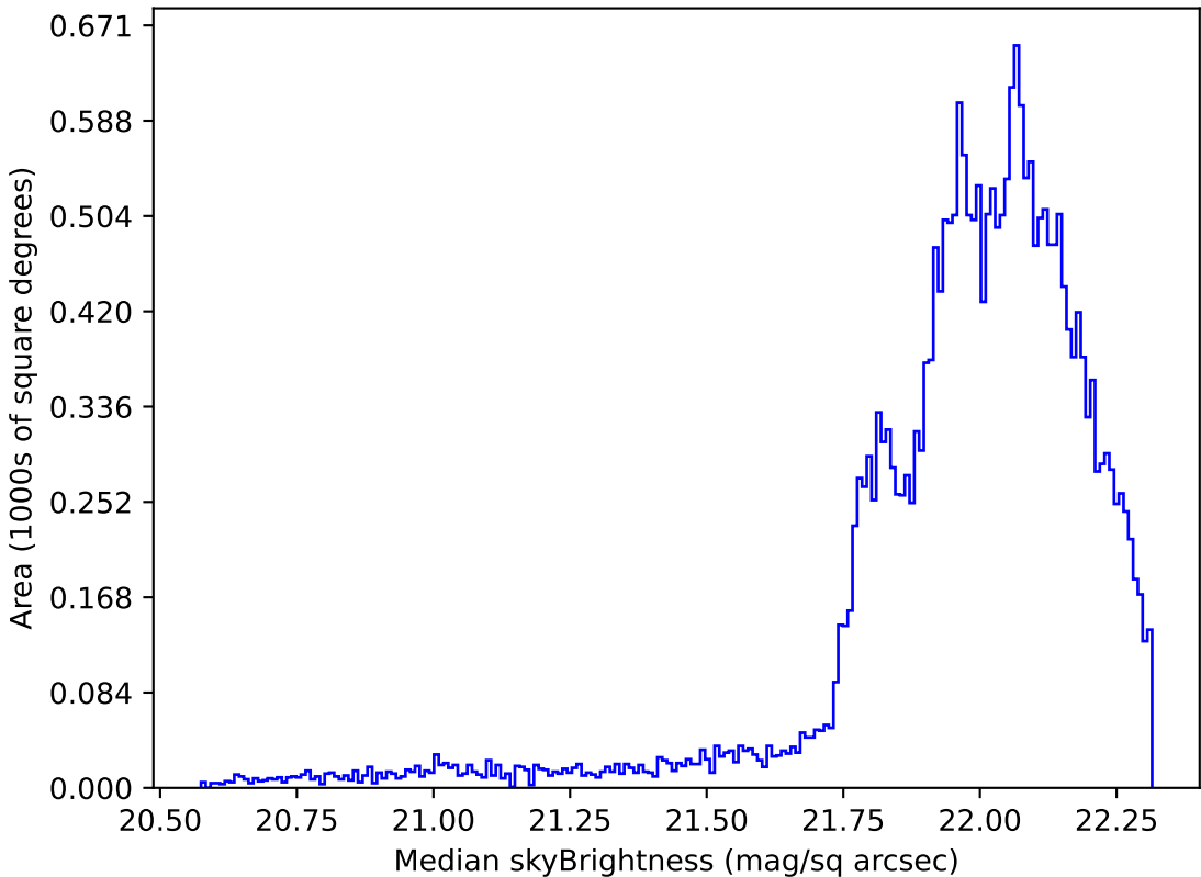
ddf_loaded_half_fl1_v3.4_10yrs Yr 1 g band: Median skyBrightness
