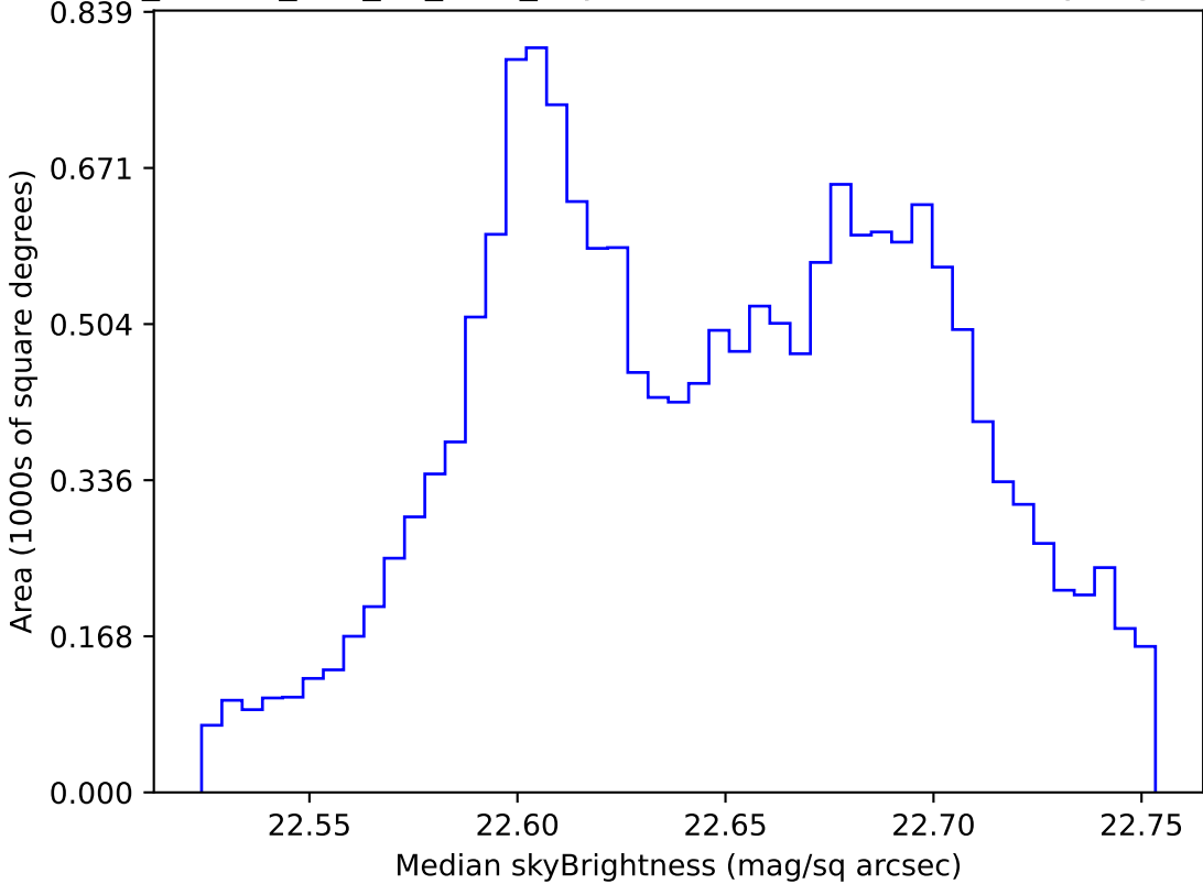
ddf_loaded_half_fl1_v3.4_10yrs WFD u band: Median skyBrightness
