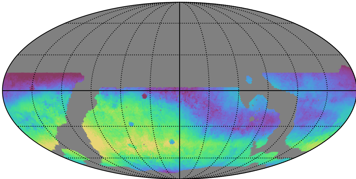
ddf_loaded_half_fl1_v3.4_10yrs WFD r band: Median skyBrightness
