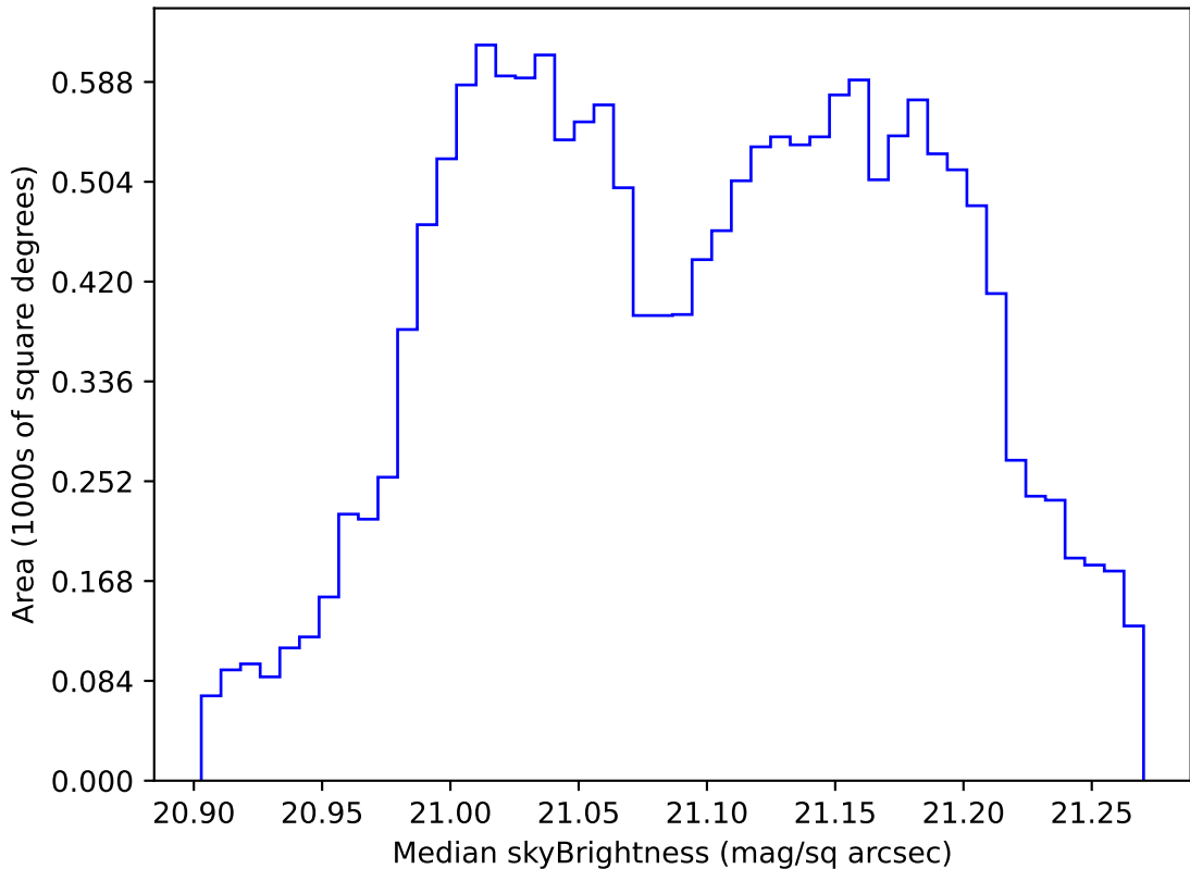
ddf_loaded_half_fl1_v3.4_10yrs WFD r band: Median skyBrightness
