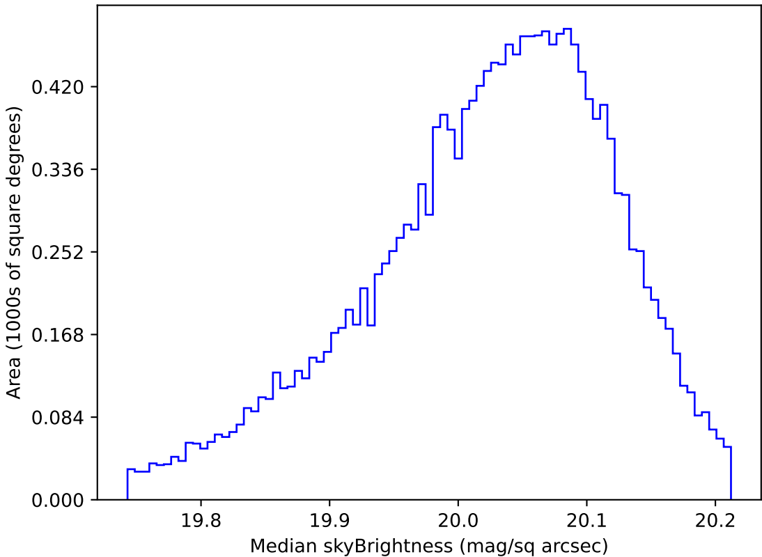
ddf_loaded_half_fl1_v3.4_10yrs WFD i band: Median skyBrightness
