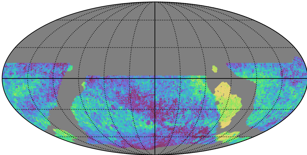
ddf_loaded_half_fl1_v3.4_10yrs WFD all bands: Median skyBrightness
