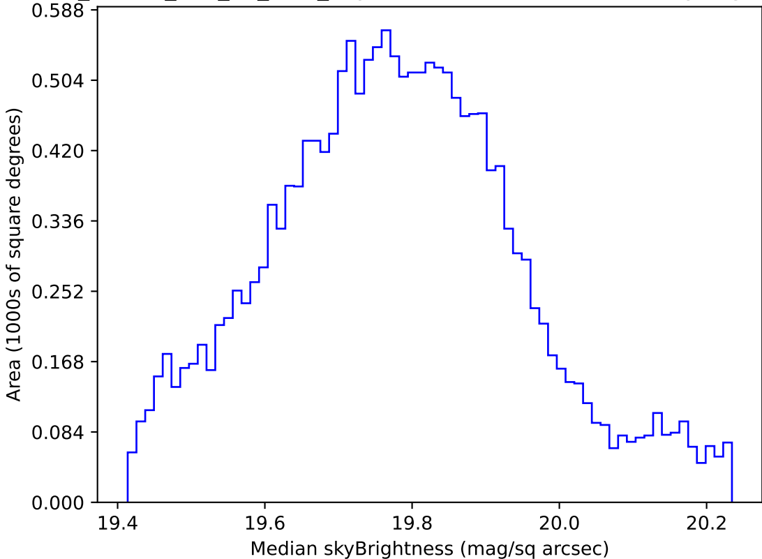
ddf_loaded_half_fl1_v3.4_10yrs WFD all bands: Median skyBrightness
