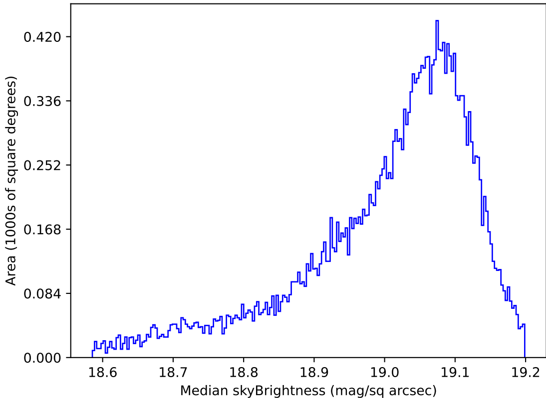
ddf_loaded_half_fl1_v3.4_10yrs All sky z band: Median skyBrightness
