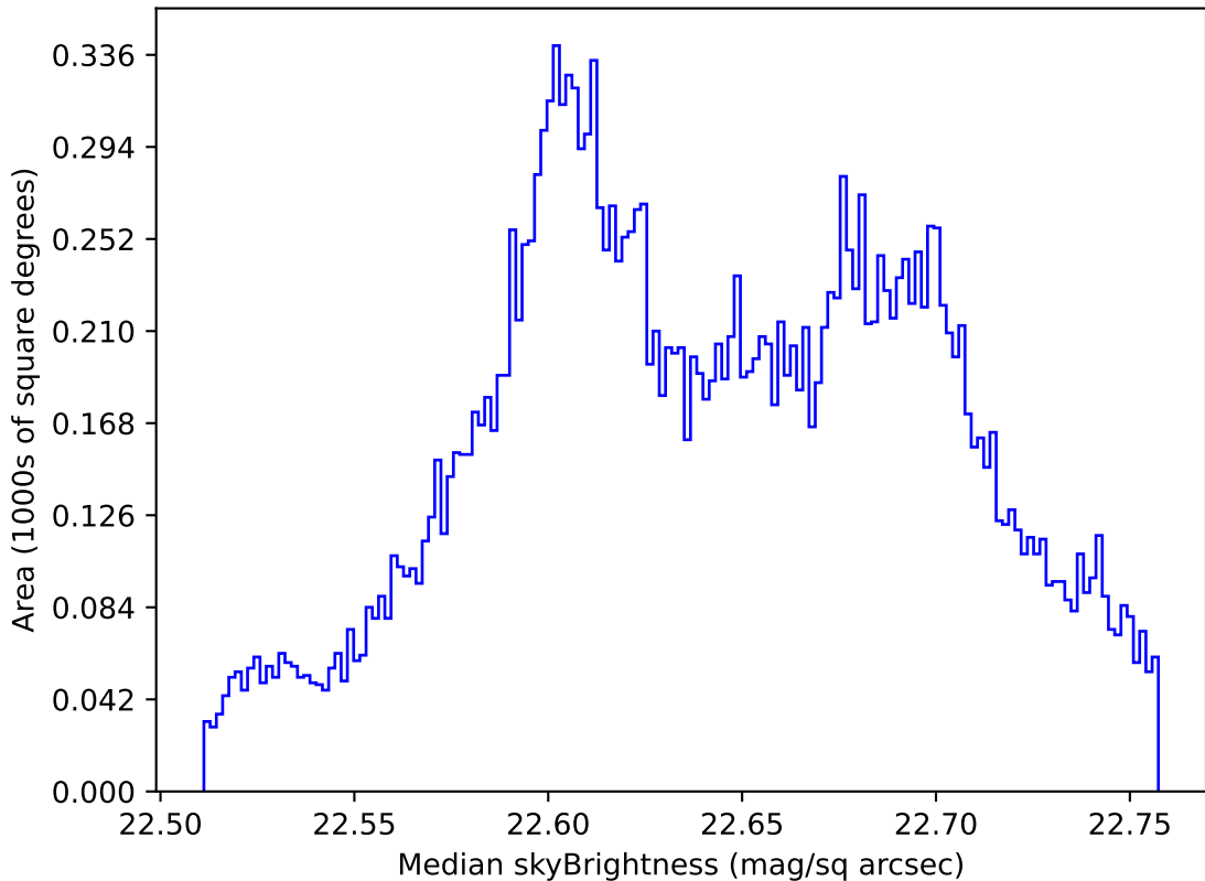
ddf_loaded_half_fl1_v3.4_10yrs All sky u band: Median skyBrightness
