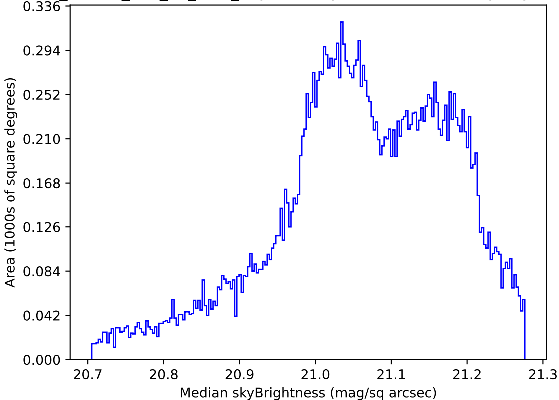
ddf_loaded_half_fl1_v3.4_10yrs All sky r band: Median skyBrightness
