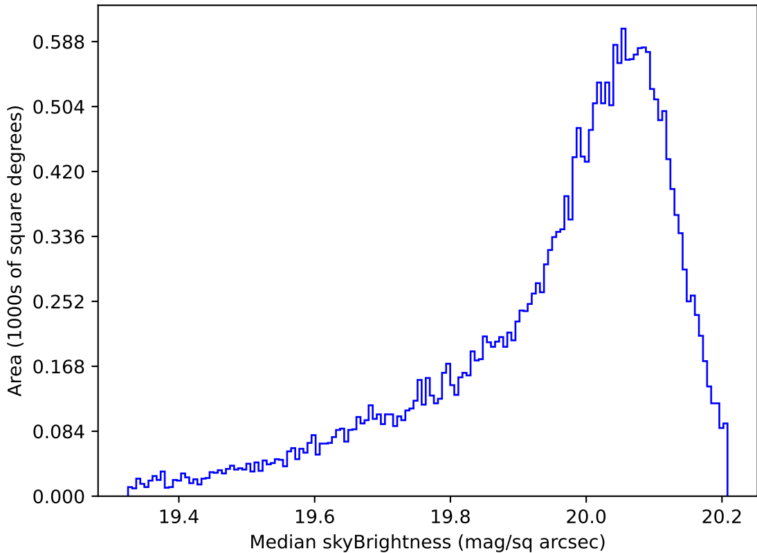
ddf_loaded_half_fl1_v3.4_10yrs All sky i band: Median skyBrightness
