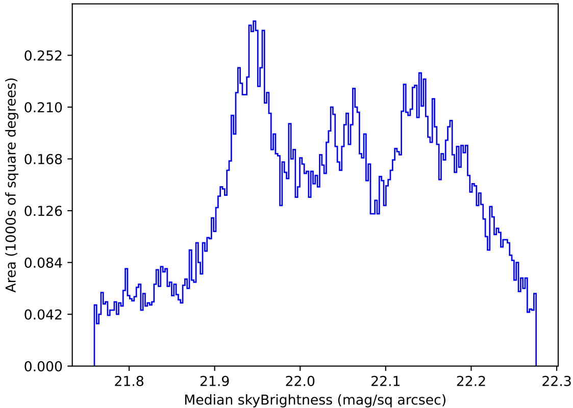
ddf_loaded_half_fl1_v3.4_10yrs All sky g band: Median skyBrightness
