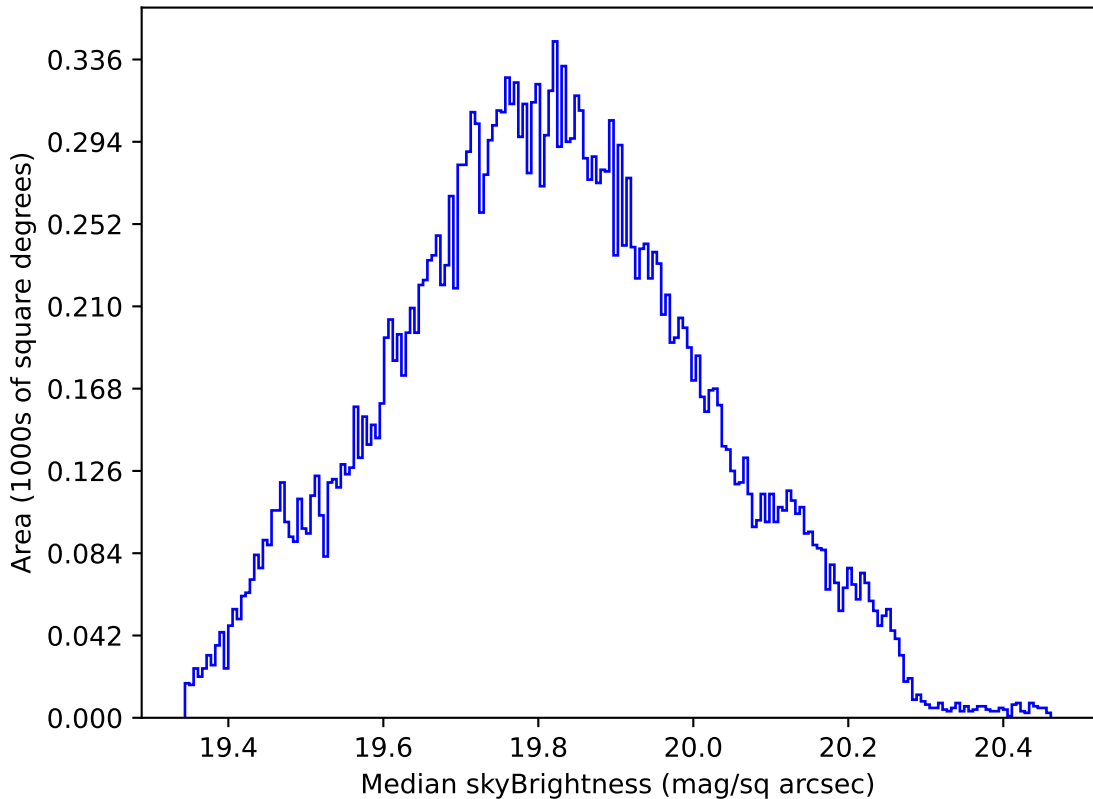
ddf_loaded_half_fl1_v3.4_10yrs All sky all bands: Median skyBrightness
