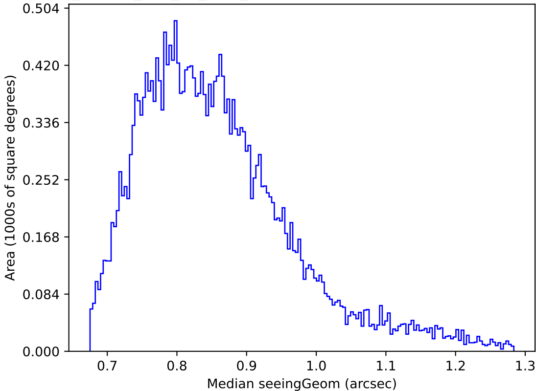
ddf_loaded_half_fl1_v3.4_10yrs Yr 1 z band: Median seeingGeom
