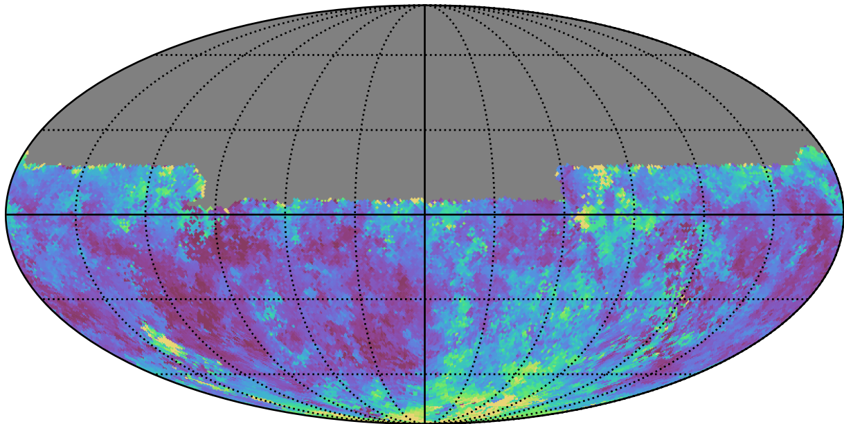
ddf_loaded_half_fl1_v3.4_10yrs Yr 1 y band: Median seeingGeom
