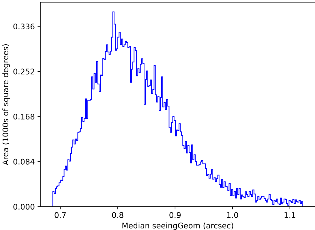
ddf_loaded_half_fl1_v3.4_10yrs Yr 1 y band: Median seeingGeom
