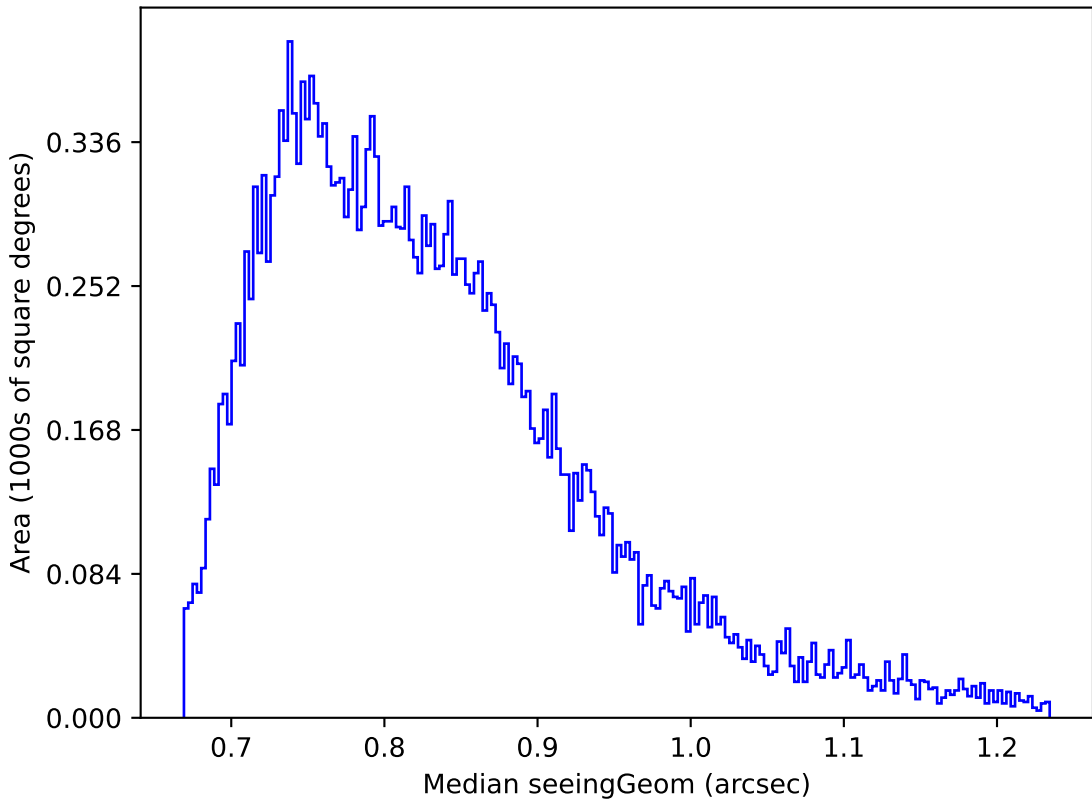
ddf_loaded_half_fl1_v3.4_10yrs Yr 1 i band: Median seeingGeom
