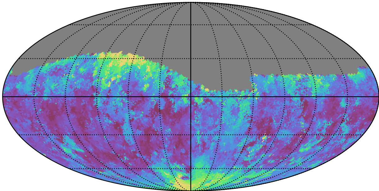
ddf_loaded_half_fl1_v3.4_10yrs Yr 1 g band: Median seeingGeom
