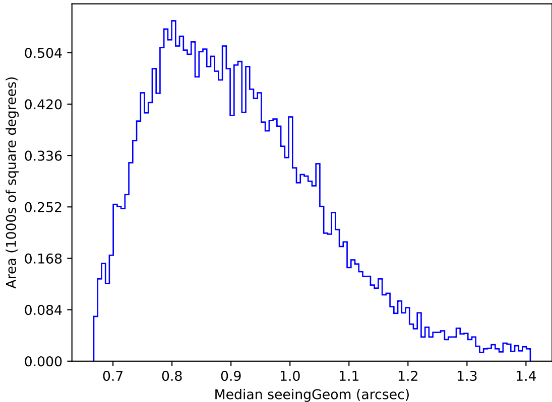
ddf_loaded_half_fl1_v3.4_10yrs Yr 1 g band: Median seeingGeom
