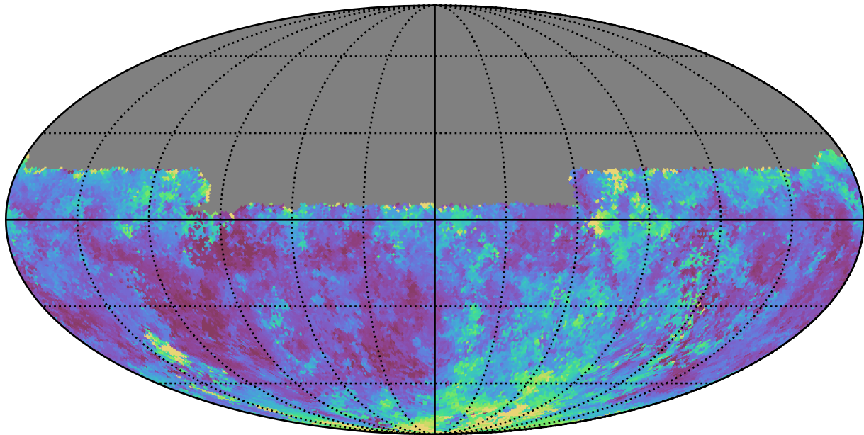
ddf_loaded_half_fl1_v3.4_10yrs Yr 1 y band: Median seeingEff
