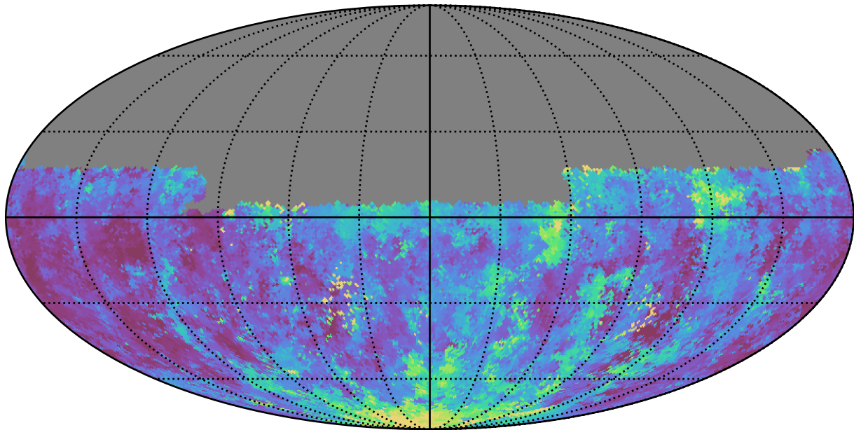
ddf_loaded_half_fl1_v3.4_10yrs Yr 1 u band: Median seeingEff
