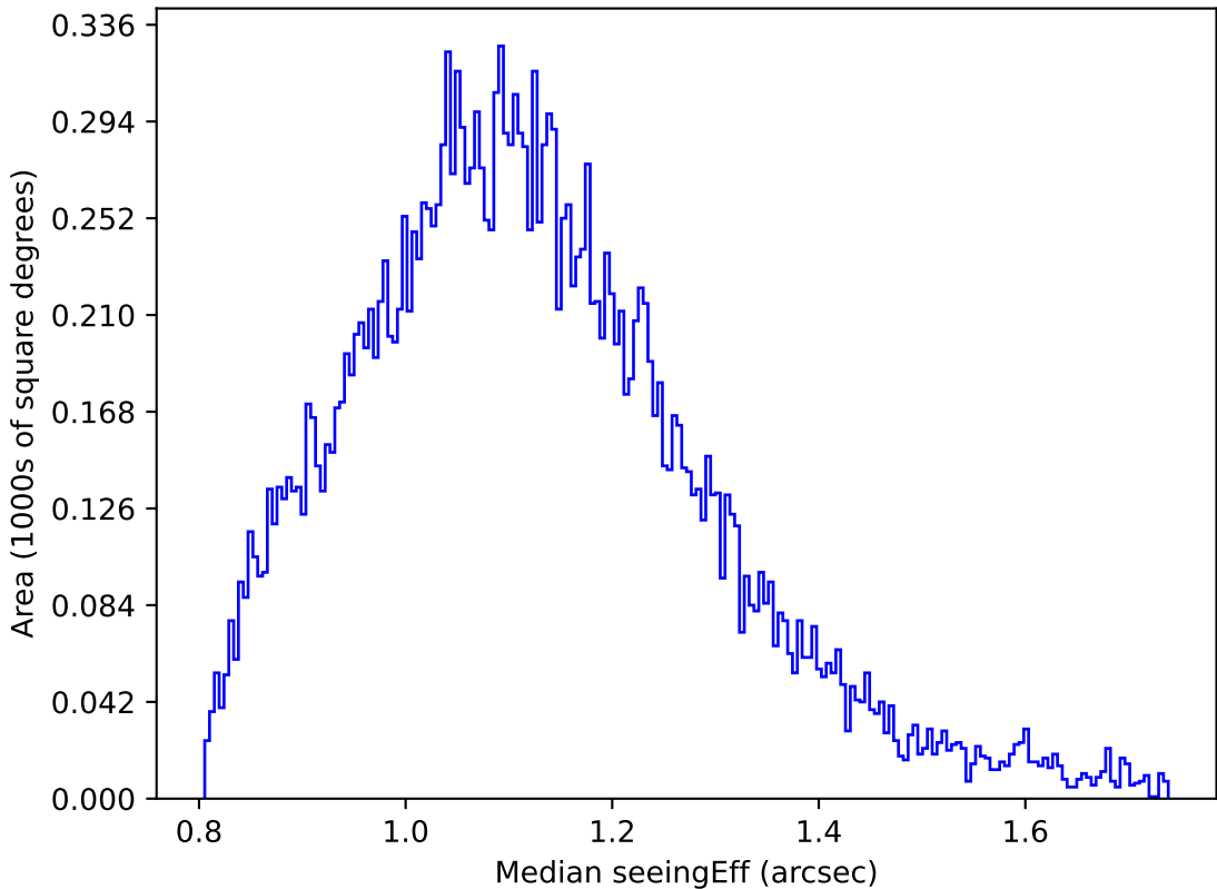
ddf_loaded_half_fl1_v3.4_10yrs Yr 1 u band: Median seeingEff
