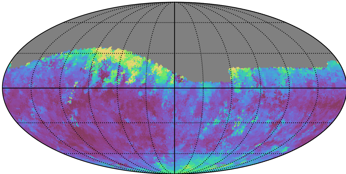
ddf_loaded_half_f11_v3.4_10yrs Yr 1 r band: Median seeingEff
