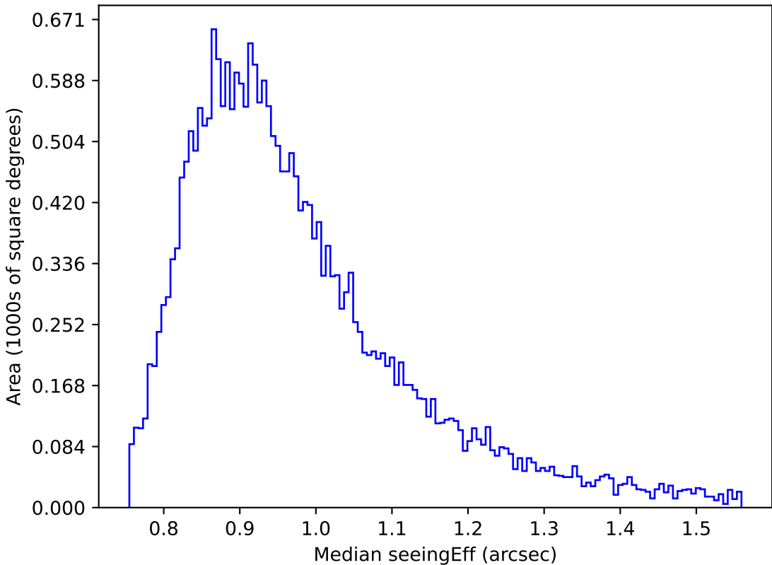
ddf_loaded_half_fl1_v3.4_10yrs Yr 1 r band: Median seeingEff
