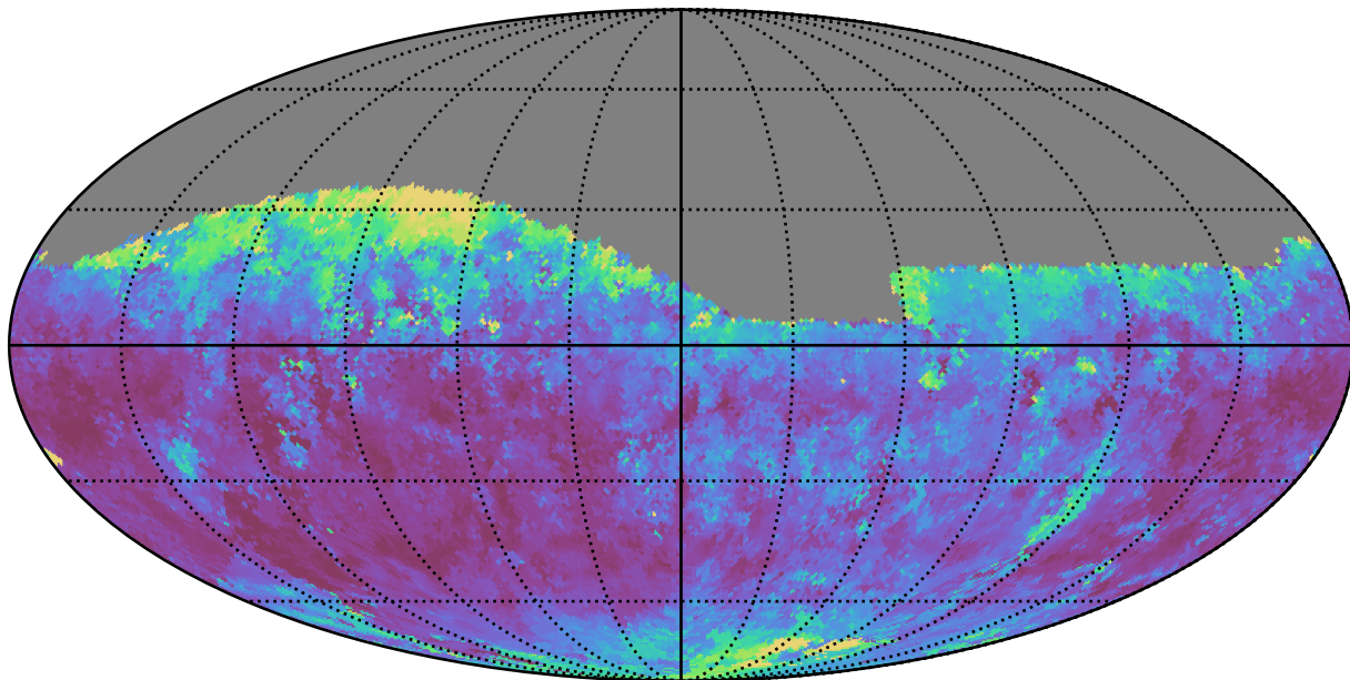
ddf_loaded_half_fl1_v3.4_10yrs Yr 1 i band: Median seeingEff
