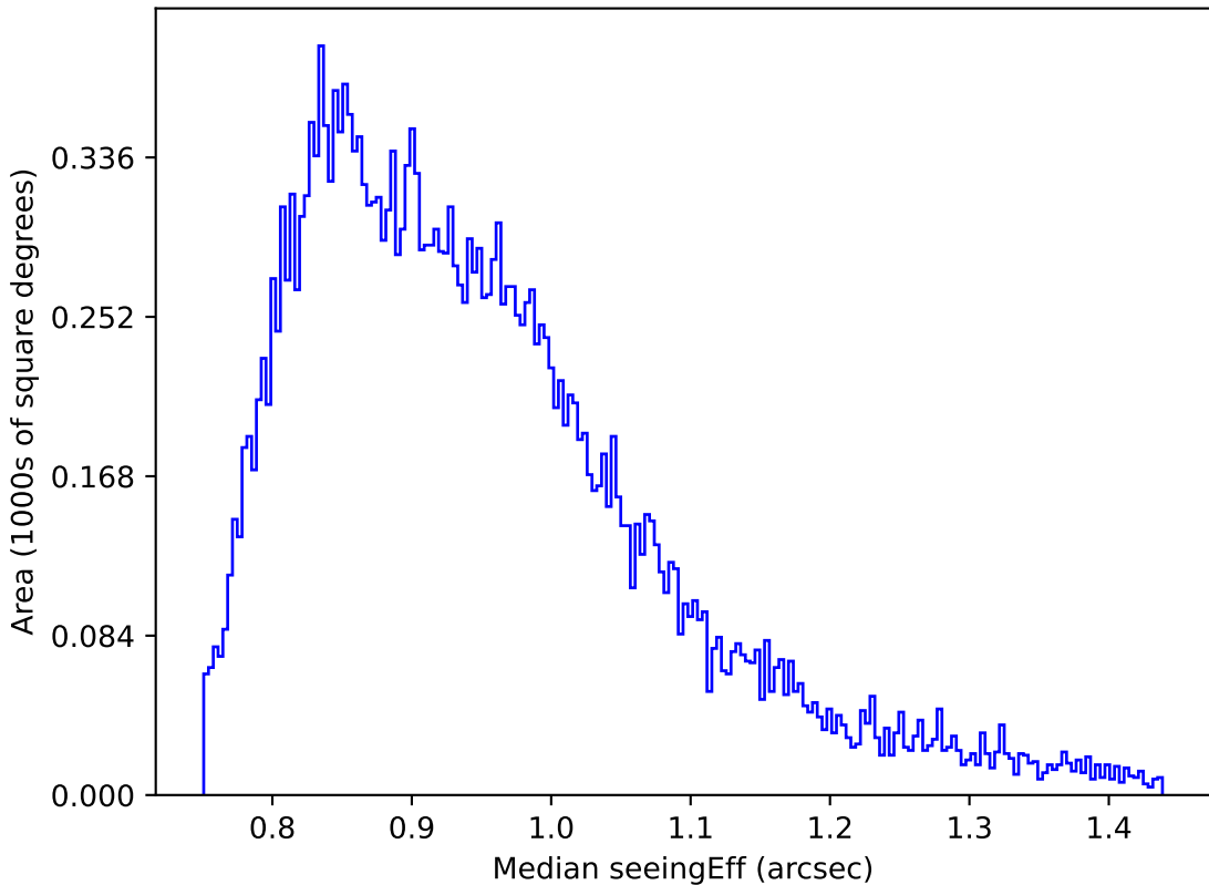
ddf_loaded_half_fl1_v3.4_10yrs Yr 1 i band: Median seeingEff
