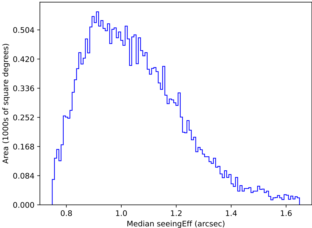
ddf_loaded_half_fl1_v3.4_10yrs Yr 1 g band: Median seeingEff
