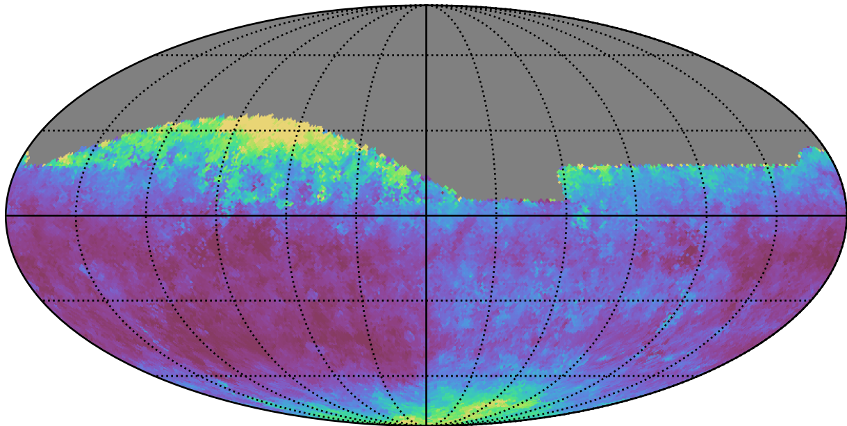
ddf_loaded_half_fl1_v3.4_10yrs Yr 1 all bands: Median seeingEff
