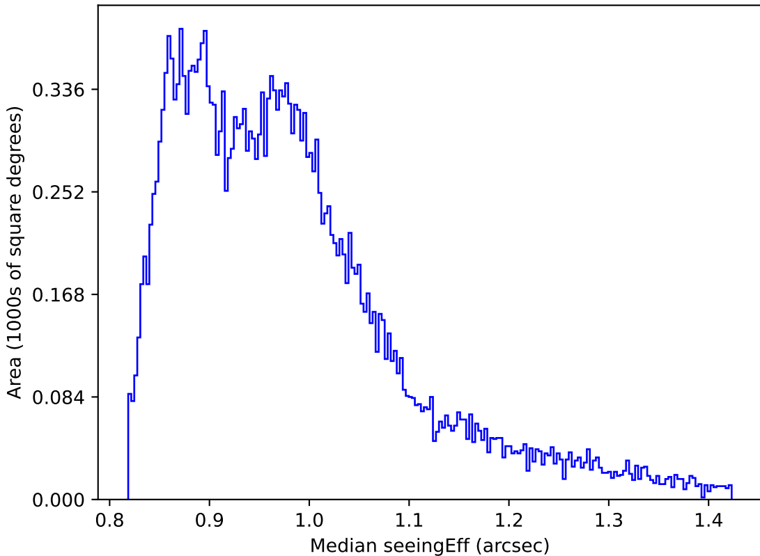
ddf_loaded_half_fl1_v3.4_10yrs Yr 1 all bands: Median seeingEff
