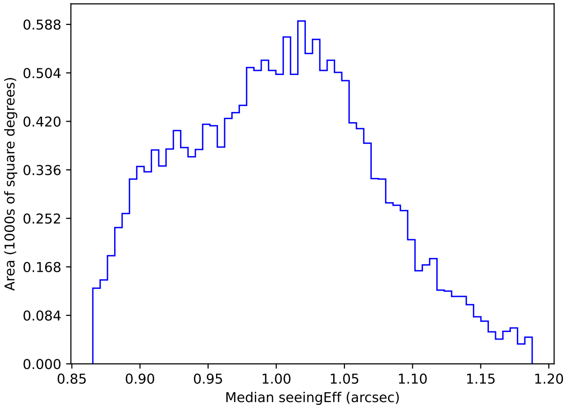
ddf_loaded_half_fl1_v3.4_10yrs WFD z band: Median seeingEff
