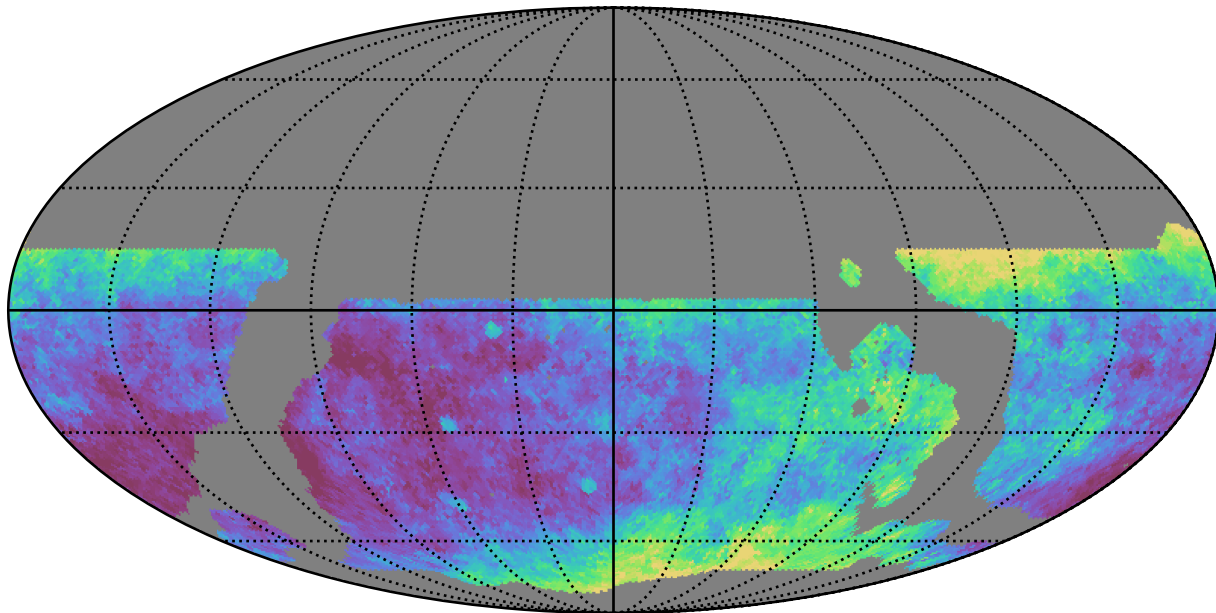
ddf_loaded_half_fl1_v3.4_10yrs WFD y band: Median seeingEff
