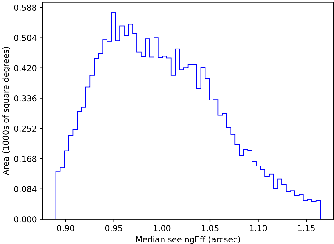
ddf_loaded_half_fl1_v3.4_10yrs WFD y band: Median seeingEff
