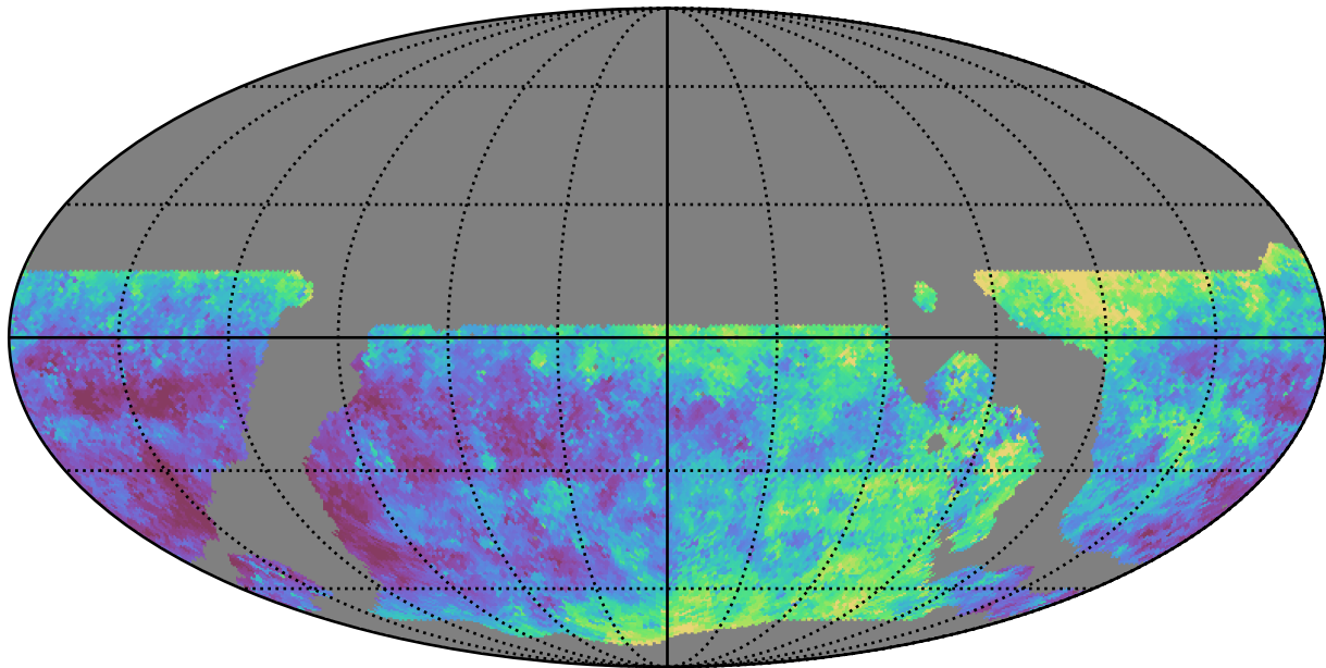
ddf_loaded_half_fl1_v3.4_10yrs WFD u band: Median seeingEff
