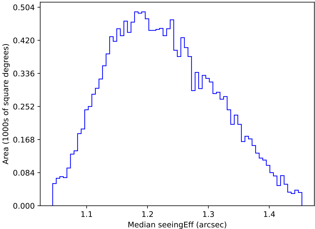
ddf_loaded_half_fl1_v3.4_10yrs WFD u band: Median seeingEff
