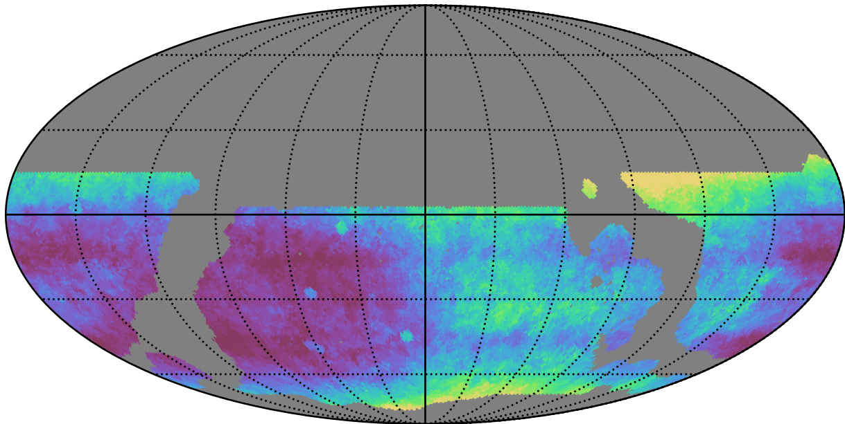
ddf_loaded_half_fl1_v3.4_10yrs WFD r band: Median seeingEff
