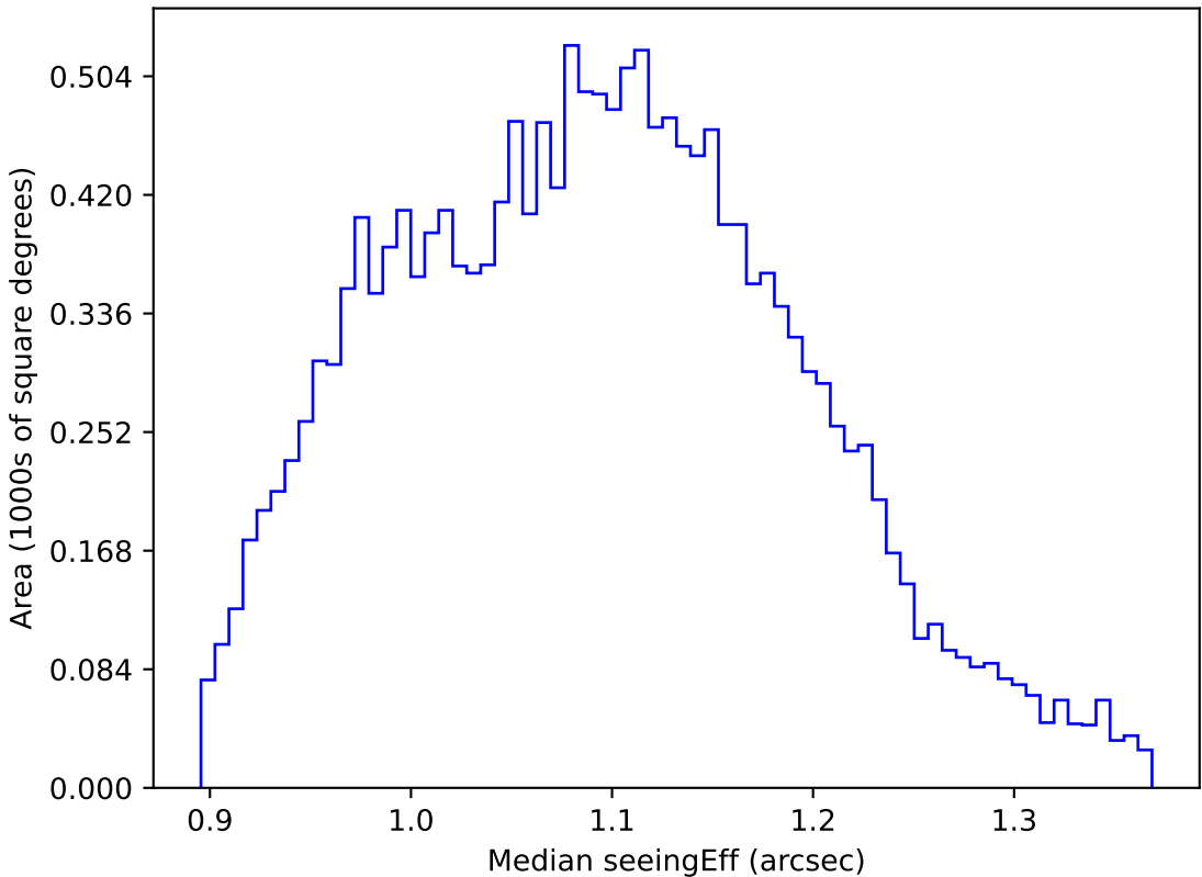
ddf_loaded_half_fl1_v3.4_10yrs WFD g band: Median seeingEff
