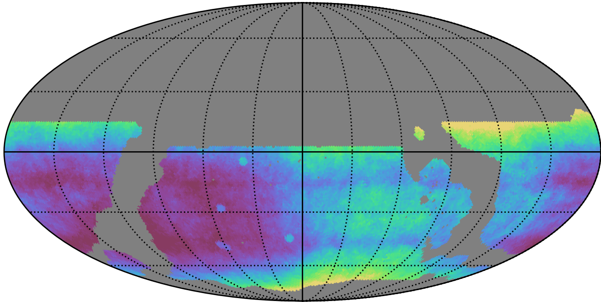
ddf_loaded_half_fl1_v3.4_10yrs WFD all bands: Median seeingEff
