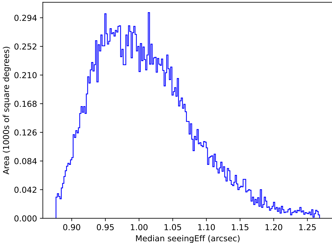
ddf_loaded_half_fl1_v3.4_10yrs All sky y band: Median seeingEff
