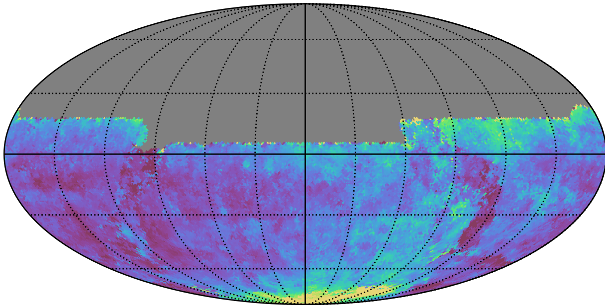
ddf_loaded_half_fl1_v3.4_10yrs All sky u band: Median seeingEff
