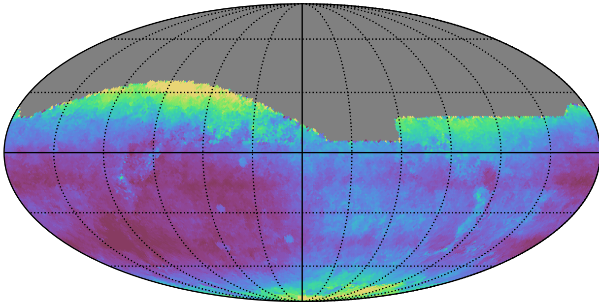
ddf_loaded_half_fl1_v3.4_10yrs All sky r band: Median seeingEff
