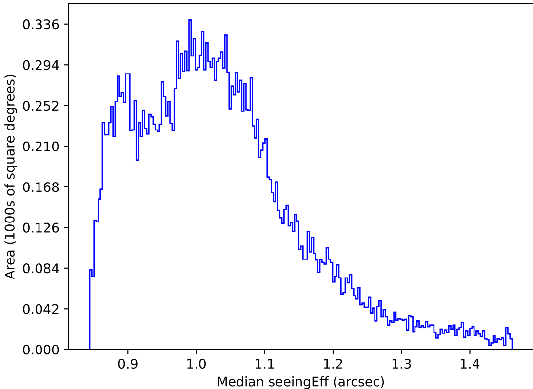
ddf_loaded_half_fl1_v3.4_10yrs All sky i band: Median seeingEff
